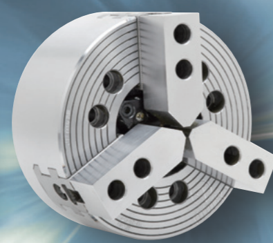
He
