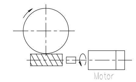
Motor 2/120 \times 1/1 = 1/60 ギア系統図 GEAR TRAIN SYSTEM DIAGRAM
